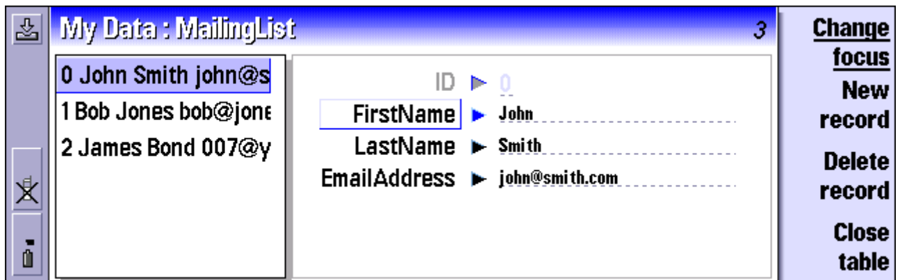
Cards view.
