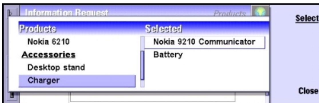
Figure 4-9 Multiple-selection list
