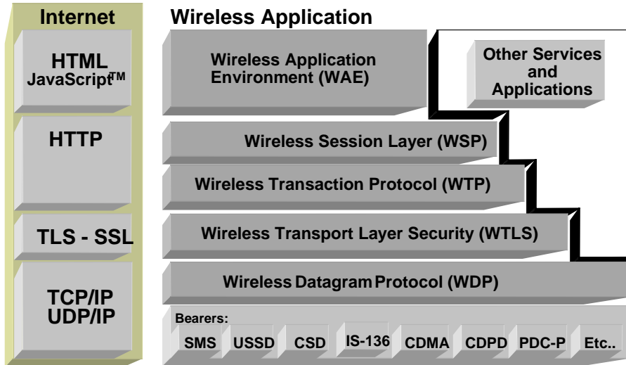
Figure 2-1 Comparison of Internet and WAP Architecture
